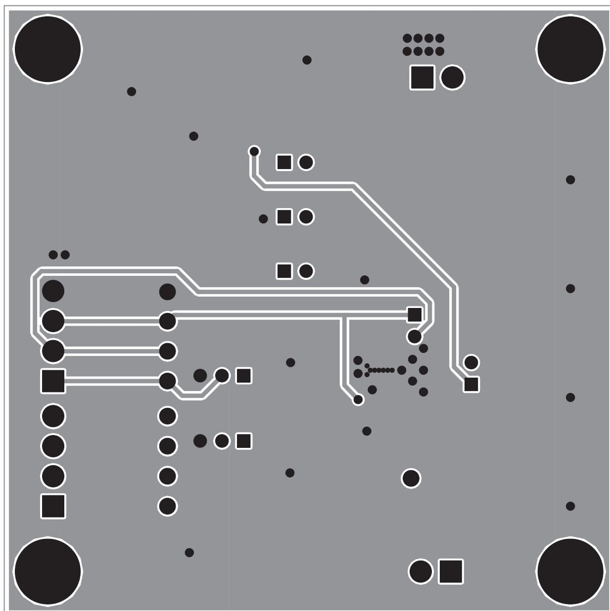
Figure 3. Bottom Layer
