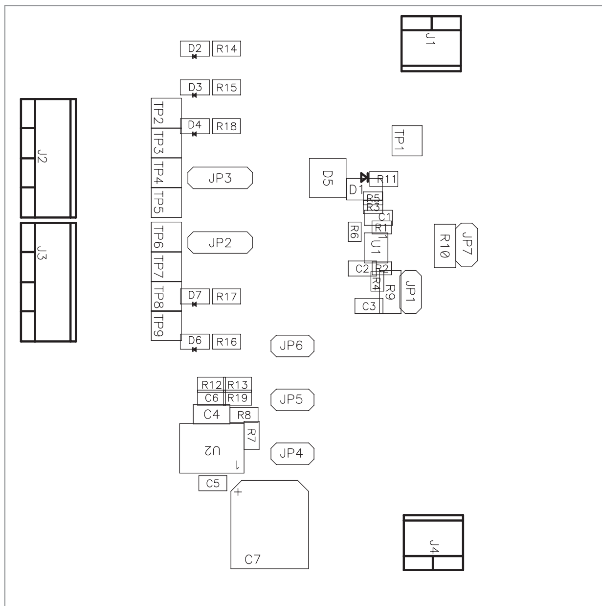
Figure 5. Top Assembly
