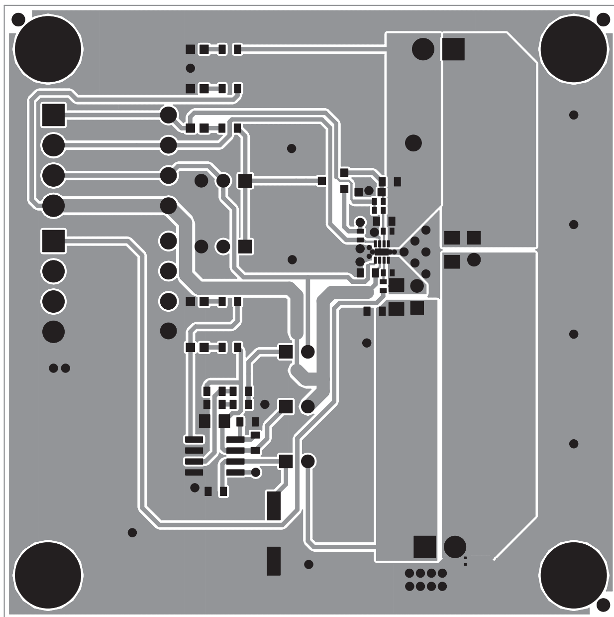
Figure 2. Top Layer
